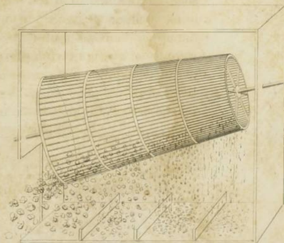
Cylinder for washing the Cascalliao.
